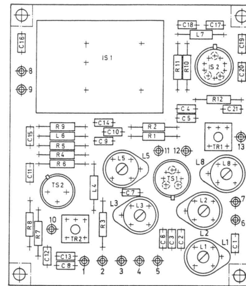
Bestückungsplan/Printed Circuit Board 52.1364.450.00
