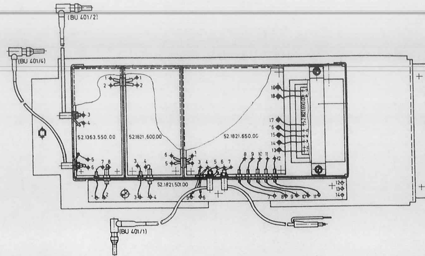
2. Oszillator 52.1821.500.00 (01)
