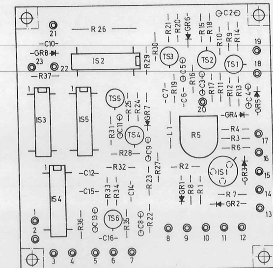
Frequenznormal 52.1821.650.00 (-)
