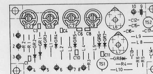
Variabler Oszillator 52.1821.251.00 (02)
