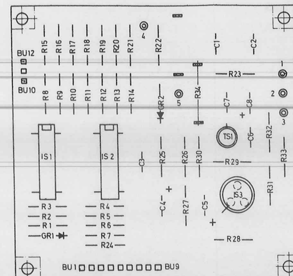
D/A-Wandler 52.1821.300.00 (01)
