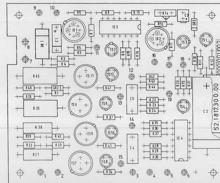
Wandler 52.1817.300.00 (01)
