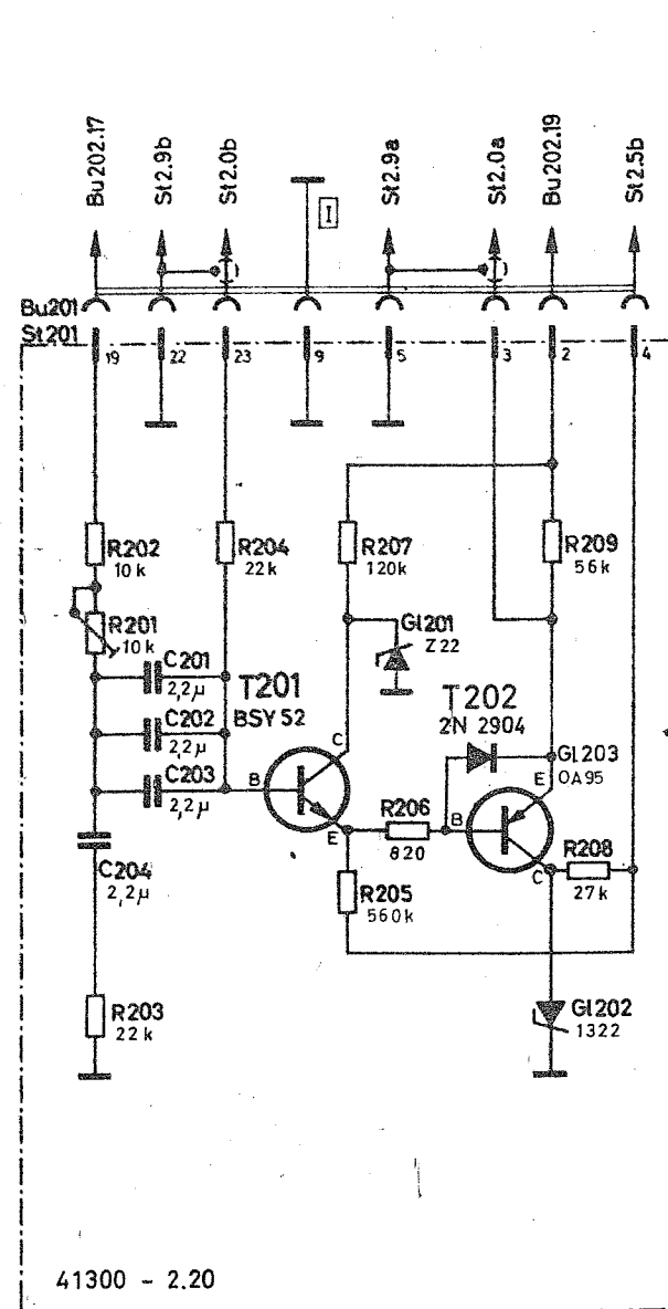
FM-Impedanzwandler
