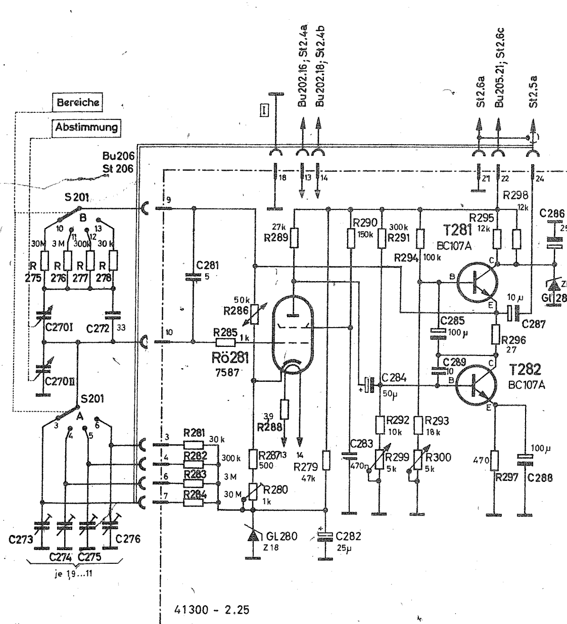
NF-Generator
